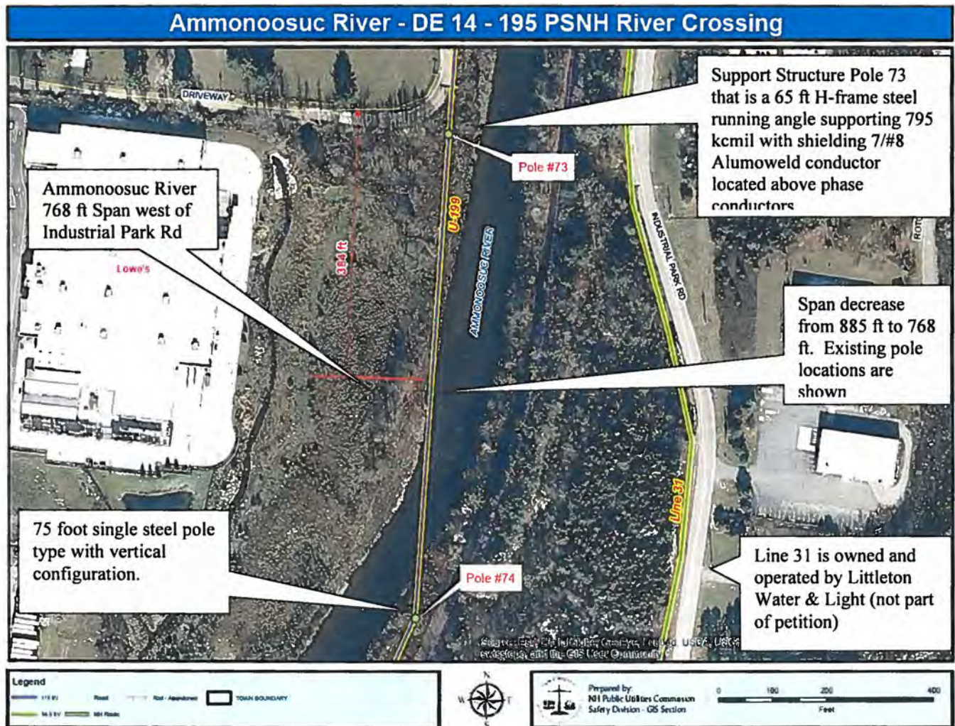
Figure 1: 115kV U199 transmission line in Littleton looking north with all the structures and spans shown.
